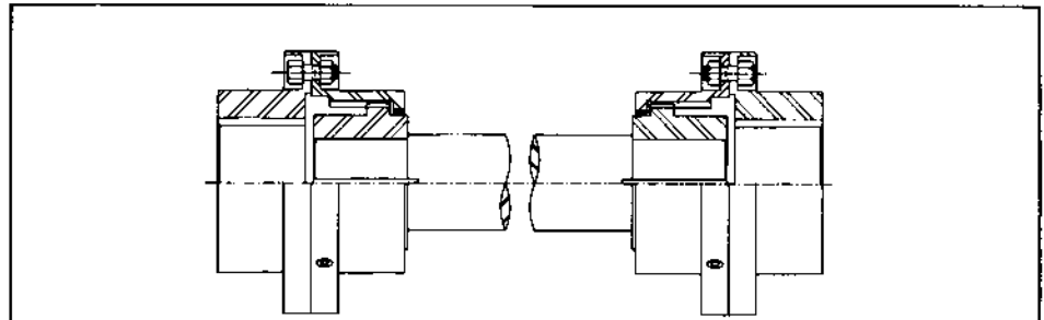
FIG. A TANDEM - FLEXIBLE HALVES ON FLOATING SHAFT
