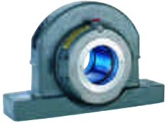
Pillow Block Unit 1 3/16" / 30mm to 24" / 600mm Available in cast iron nodular iron or steel
