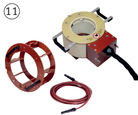
⑪ HEAT-INDUCTOR
