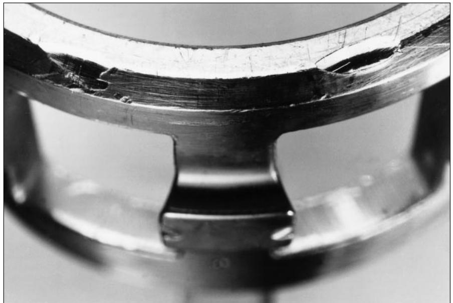
95: Metal cage with dents
