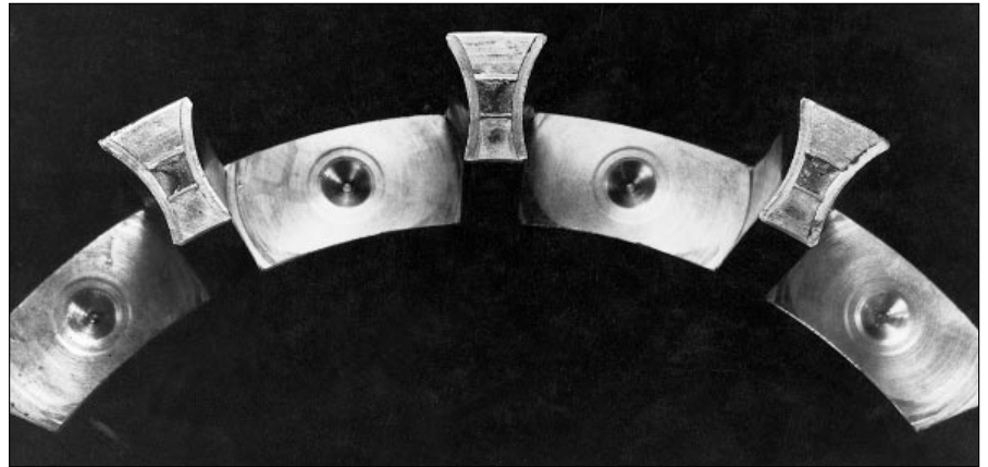
92: Fractured cage-rivet connections may result from vibration stress.
