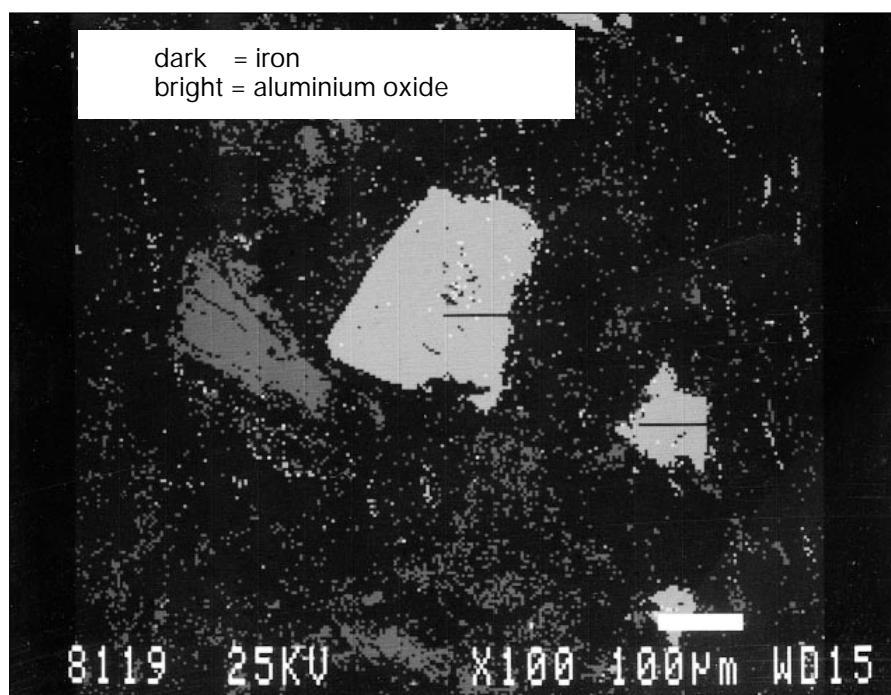
113 b: Material composition of foreign particles
