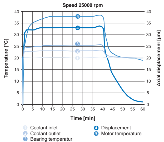
The diagram illustrates the axial shaft growth of a spindle operating at 25000 rpm.
