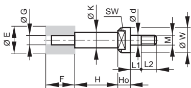
Type 4: Quill with nut (MU)
