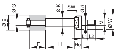
Type 4: Quill with nut (MU)
