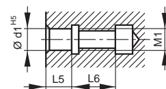
Close-fit hole for type 2 and 3
