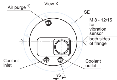
straight "GA" style electrical connector 1)
