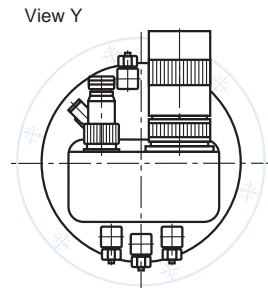
with angled "MAC" style electrical connector 1)
