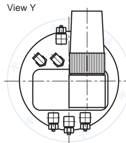
with angled "GA" style electrical connector 1)
