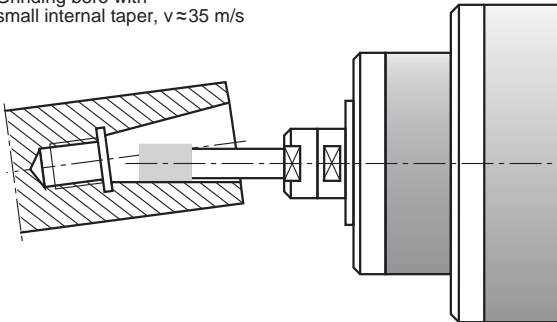
Grinding bore and conical seating in fuel injector, v \approx 35 m/s
