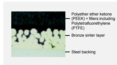
Fig. 1: Hi-eX-microsection
