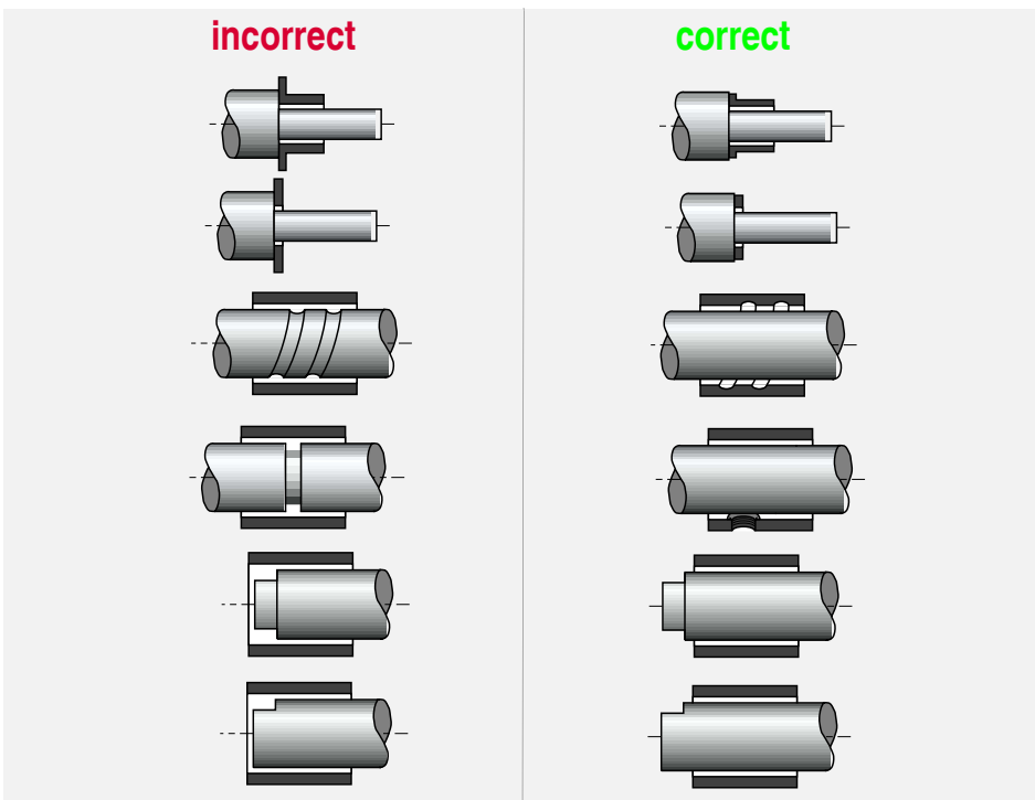
Fig. 25: Counterface design
