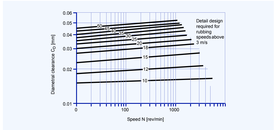
Fig. 23: Hi-eX minimum clearances - bush diameters D_i 10-50 mm
