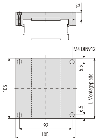
Montageplatte M Mounting plate M
