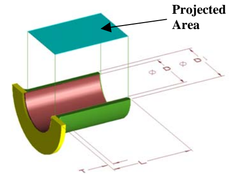
Figure 4, (Flanged Journal)
