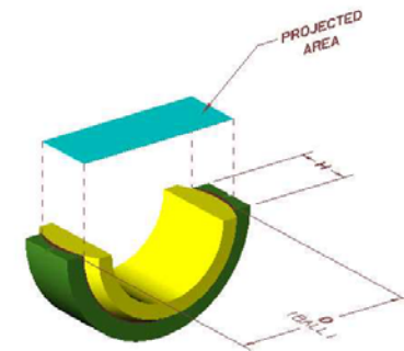
Figure 2, (Spherical Bearing Projected Area)
