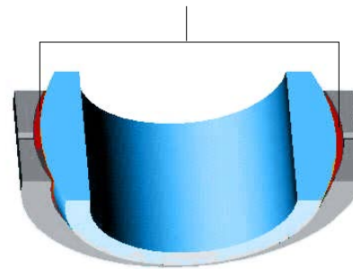
Figure 1 Cathedral Cavity
