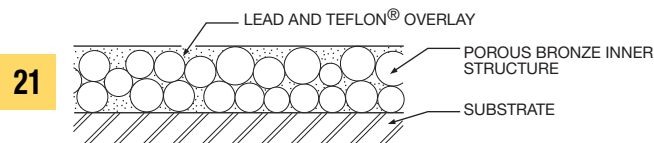
Metallic-Backed Composite Construction
