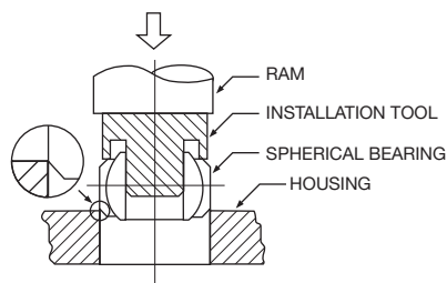
40 Spherical Bearing Installation
