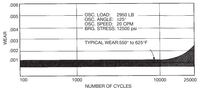
25 Typical performance of the HT liner system (oscillation under radial load, wear vs. life)
