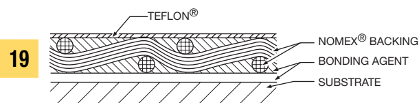
Laminate Construction
