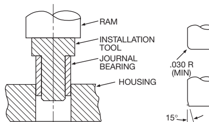
41 Sleeve Bearing Installation
