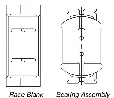
29 Lube Groove Size and Depth Exaggerated for Clarity
