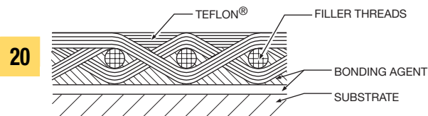
Woven Construction
