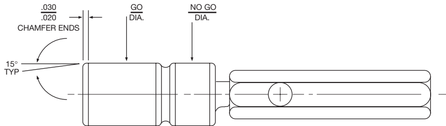
27 Plug Gage
