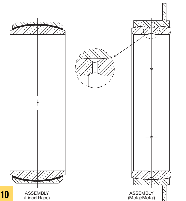
Snap-Assembled Bearings
