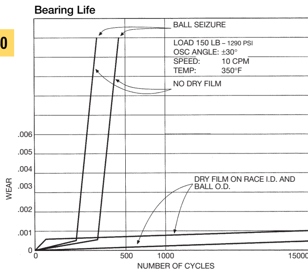
Dry Film Lubricated vs. Non-Lubricated Bearings
