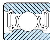
Figure 3. Two "D" Seals (contact rubber)
