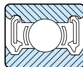
Figure 6. Two "SSD21" Seals (labyrinth design seal)
