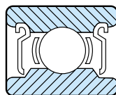
Figure 2. Two "H" Shields (non-removable)
