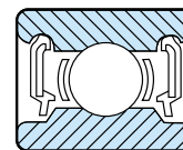
Figure 4. Two "S" Seals (non-contact rubber)
