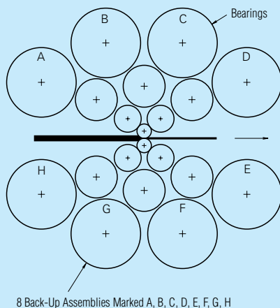
Roll Arrangement of a 20-high Sendzimir Mill
