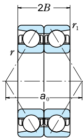
Back-to-Back DB
