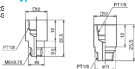
Fig-7 SF Type
