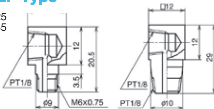
Fig-6 LF Type
