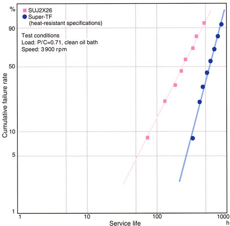
Fig. 15 Service life of 6206 ball bearings at 160°C under clean lubrication
