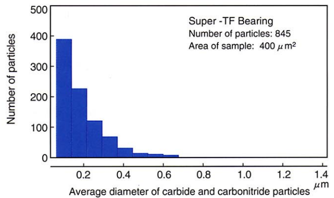
Fig. 7 Average diameter of carbide particles in an ordinary carburized steel bearing
