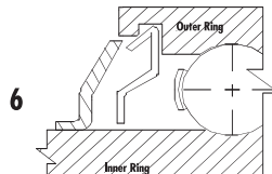
6 Z-Shield/Slinger Full cover metal shroud with slinger.
