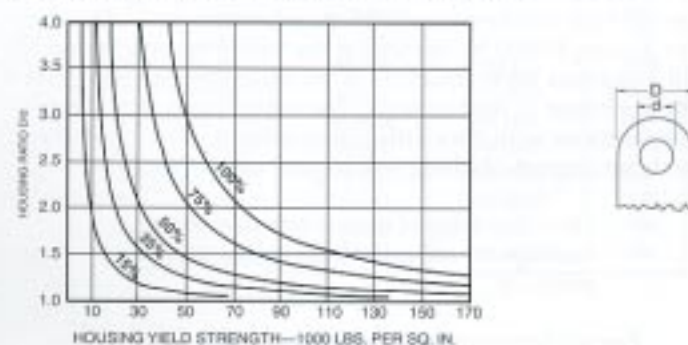
Figure 17: Influence of Housing Design on Bearing Capacity
