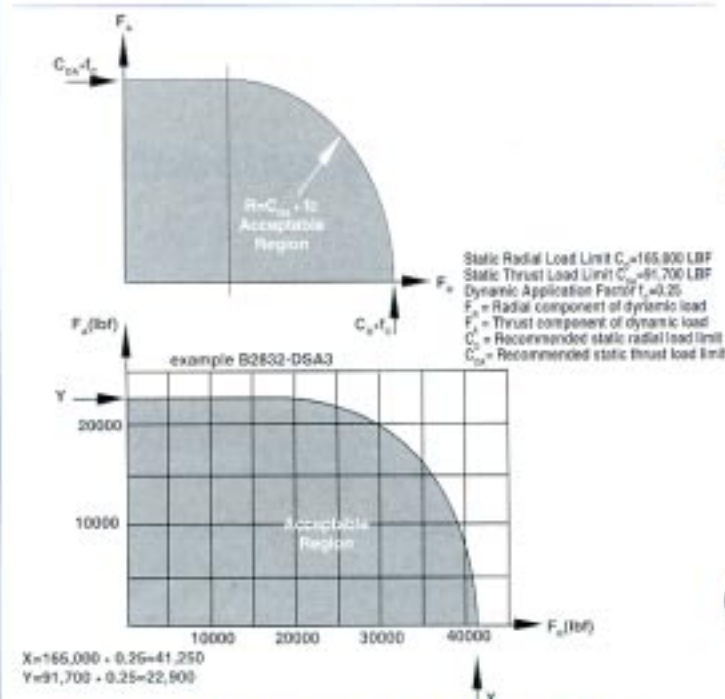
Fig. 15: Angular Contact Bearings, Double Acting
