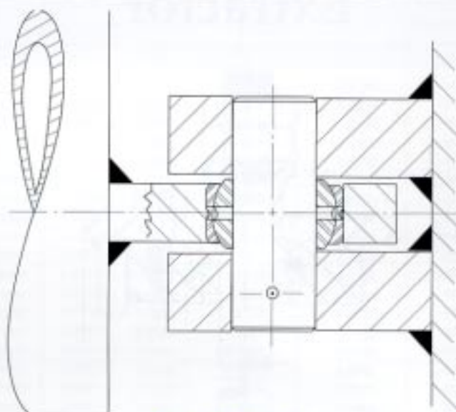
Tilt Cylinder
