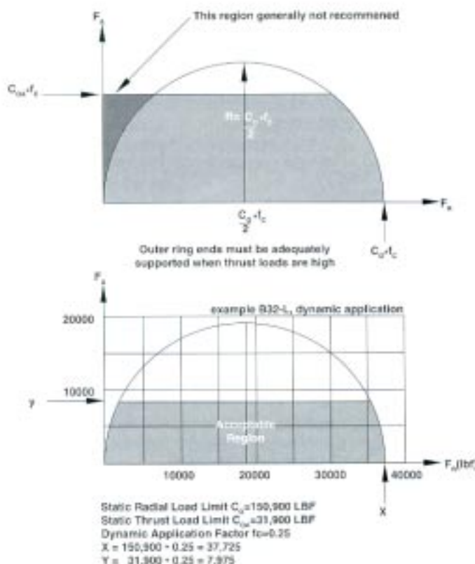
Figure 13: Radial Bearings
