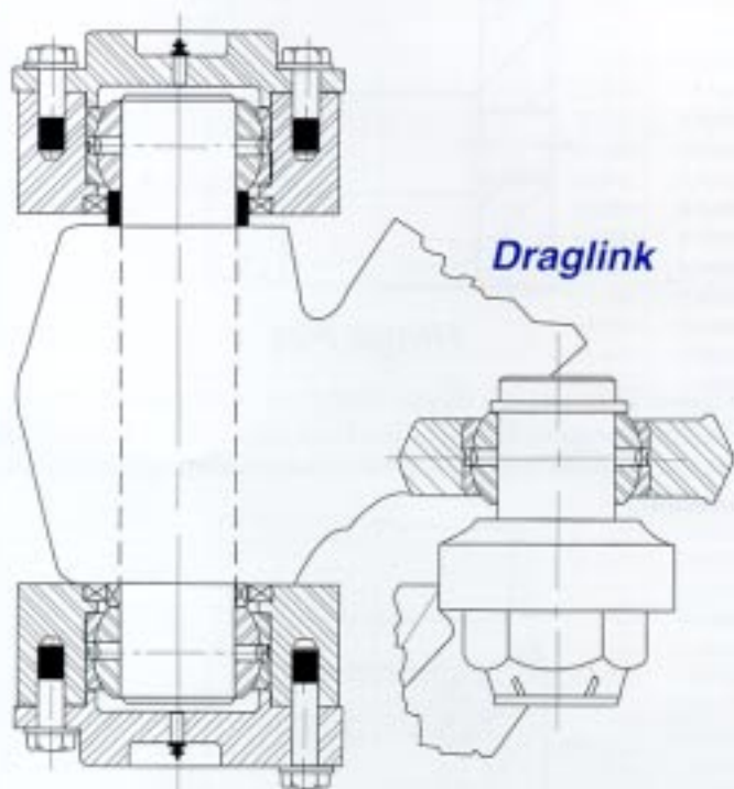
King Pin
