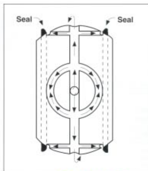
RBC QUADLUBE™ Spherical Plain Bearing
