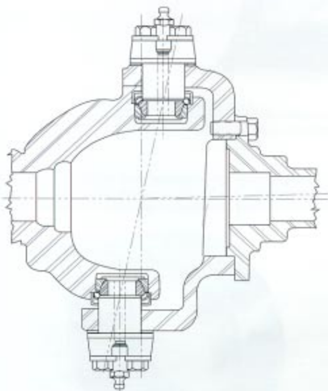
King Pin
