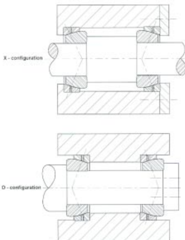
Figure 10: Bearing Arrangement
