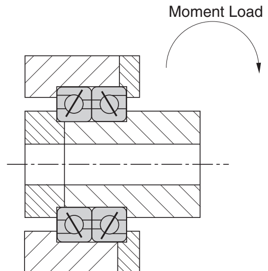
B-Type Configuration
