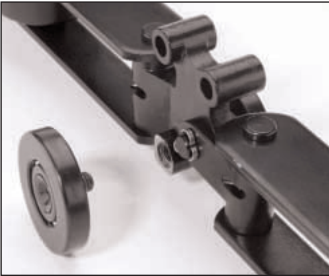
Innovative option to remove wheel for replacement. Part # 101-61259-1 for both 1295 and 1296 styles.
