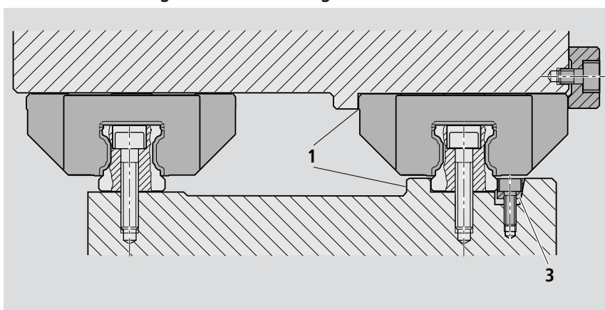
Mounting with fixation of a guide rail and runner block
