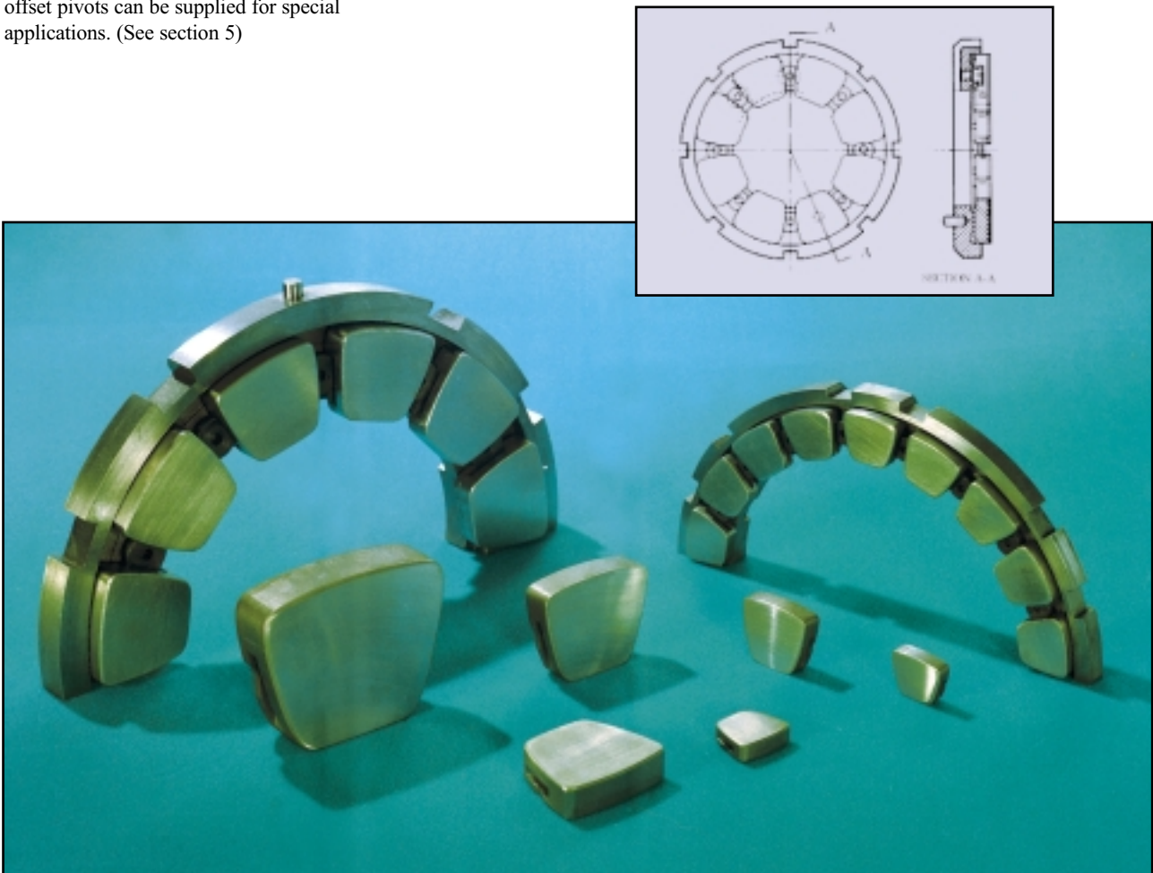
Fig 1. Standard MS Series thrust bearings in halves, and (inset) Series 8 one piece thrust bearing.
