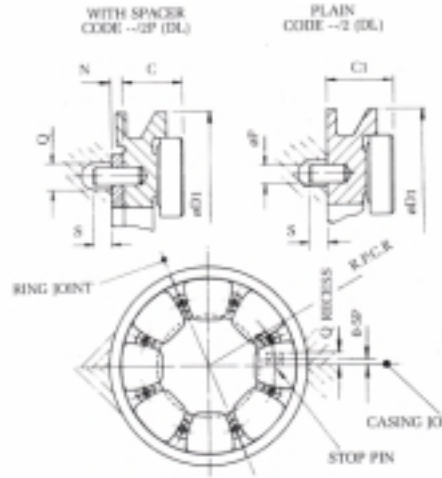
RING IN HALVES Directed Lubrication
