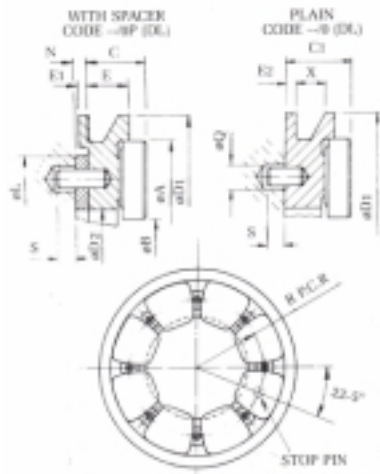
ONE PIECE RING Directed Lubrication
